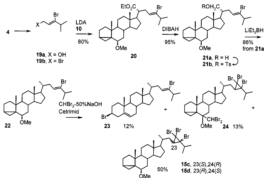
Scheme 5. Improved synthesis of calysterols 2a and 2b
