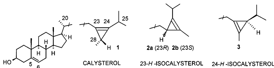
Figure 1. Structures of isomeric calysterols isolated from sponges Calyx niceaensis and Calyx podatypa
