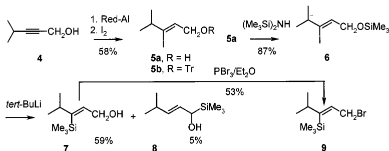
Scheme 2. Synthesis of the side chain building block 9
