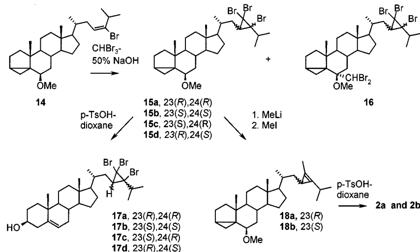
Scheme 4. Synthesis of calysterols via the vinyl bromide derivative 14
