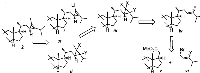
Scheme 1. Retrosynthetic analysis of compounds 2
