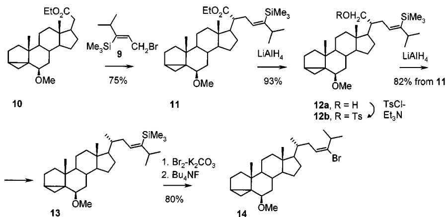
Scheme 3. Attempted synthesis of calysterols via the vinylsilane derivative 13
